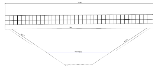
Snit F-F
