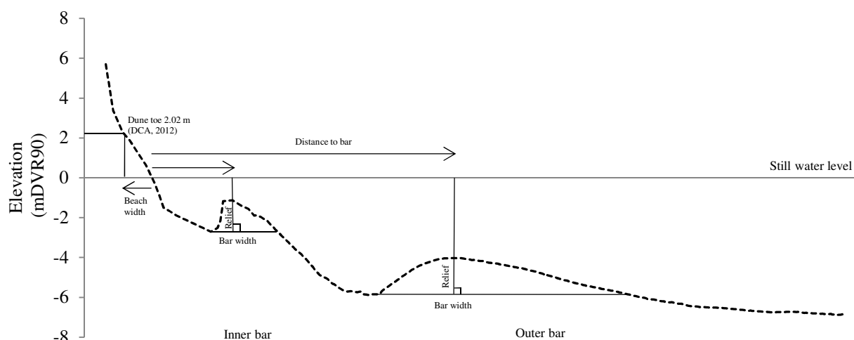
Figure 5.1: Method for analyzing coastal morphology e.g. dimensions of bars, beach and dunes
