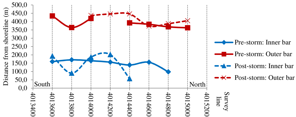
Figure 5.8: Distance from shoreline for inner and outer bars before and after storm period
