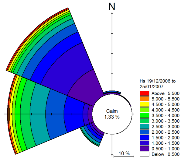
Figure 6.2: Offshore wave climate at Nymindesgab wave buoy from 19/12/2006 to 25/01/2007
