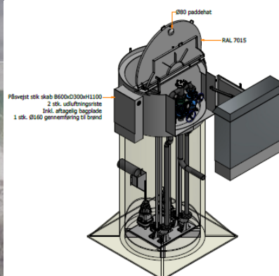
Pumpebrønd
