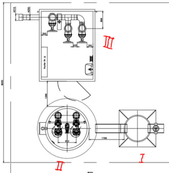
Plantegning af ny pumpestation
