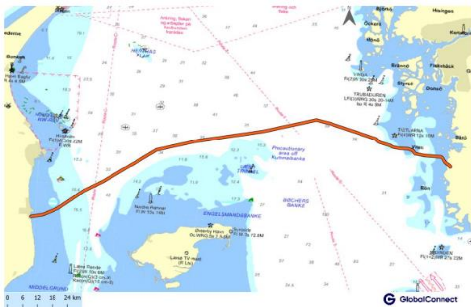
Figure 1 Planned Cable route between Seaby in Denmark and Lerkil in Sweden. The corridor 100-150 meters for surveying will be around the red line presented on the map.
