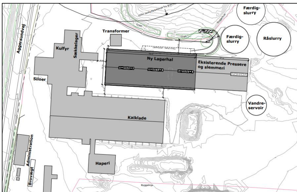
Situationsplan viser ny bygning.
